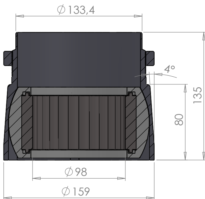
SECTION A-A SCALE 1 : 2.5
