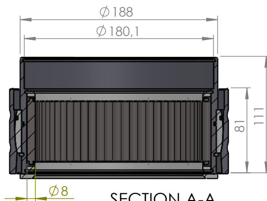
SECTION A-A SCALE 1 : 3.5
